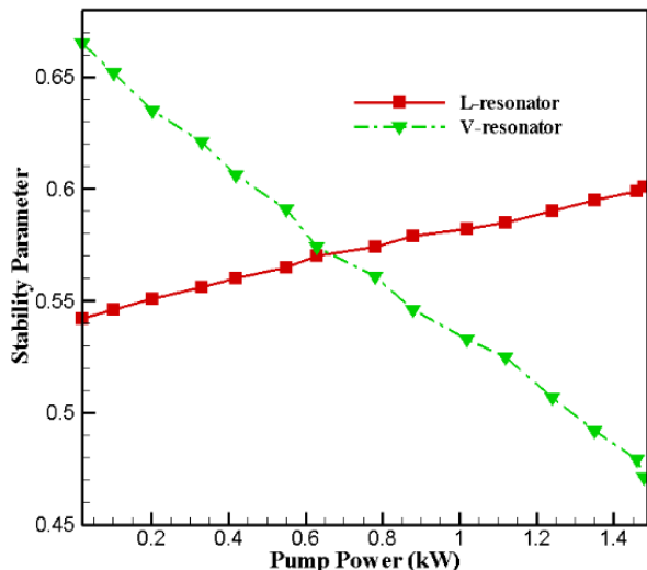
Fig. 8. Stability parameter of the designed resonators versus pumping power.
