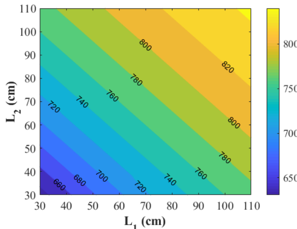
Fig. 10. TEM 00 mode spot sizes (in \mu\text{m} ) of the dumped cavities for L-shaped resonator.
