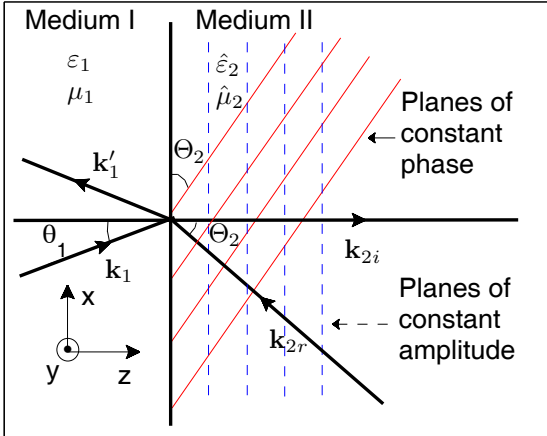
Fig. 1 (Color online) Refraction into a lossy DNG material. The planes of constant phase are perpendicular to the propagation direction and make a negative angle \theta_2 with the interface, but the planes of constant amplitude are parallel to the interface.
