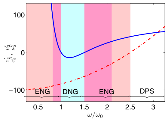
Fig. 5 (Color online) The plot of \epsilon'_2/\epsilon''_2 and \mu'_2/\mu''_2 as a function of normalized frequency \omega/\omega_0 for a lossy metamaterial described by Eqs. (17) and (18) with \omega_{ep} = 10\text{GHz} , \omega_0 = 4\text{GHz} , F = 0.56 and \gamma_e = \gamma_m = 0.01\omega
