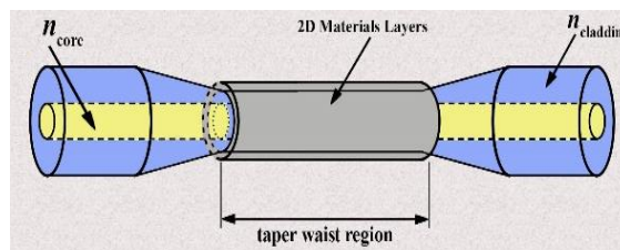
Fig. 3. The proposed FMF for temperature and strain sensing.
