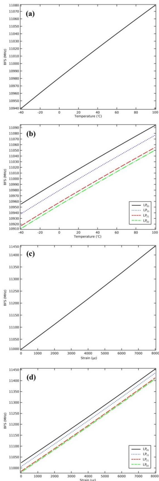
Fig. 2. BRS vs. temperature for (a) SMF and (b) FMF and strain for (c) SMF and (d) FMF at 1550 nm.
