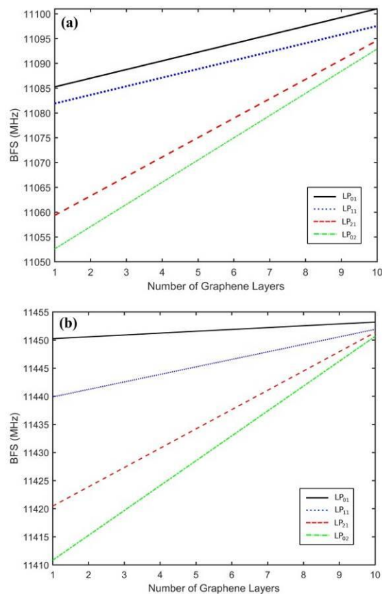
Fig. 6. Investigation of the effect of different layers of graphene on the BFS as functions of (a) temperature (at 100 °C), and (b) strain (for 8000 \mu\epsilon ), for different propagating modes.
