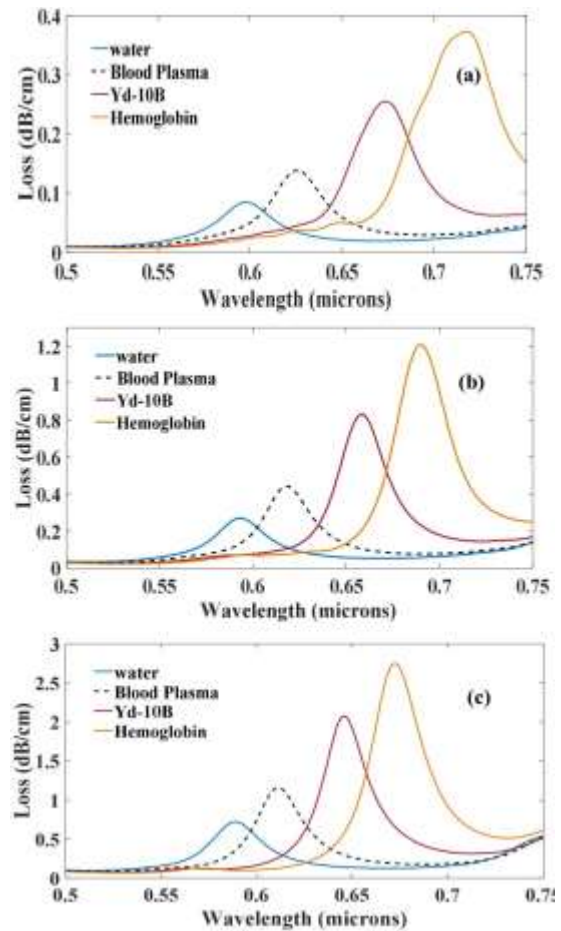
Fig. 6. The confinement loss spectra with different sensing layers and different pitch sizes \Lambda = (a) 1.9\mu m (b) 2\mu m (c) 2.1\mu m . The other parameters are d = 1.4\mu m , and d_{Au} = 45nm .
