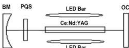
Fig. 2. Schematic of the Q-switched LED-pumped Ce:Nd:YAG laser oscillator.
