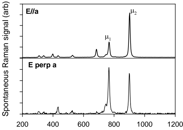
Fig. 5 Spontaneous Raman spectra for KGW for pump propagation along the N_p axis and polarization aligned parallel and perpendicular to the crystal a-axis. Two strong Raman modes are observed at h\mu_1=768\text{cm}^{-1} and h\mu_2=901\text{cm}^{-1} .
