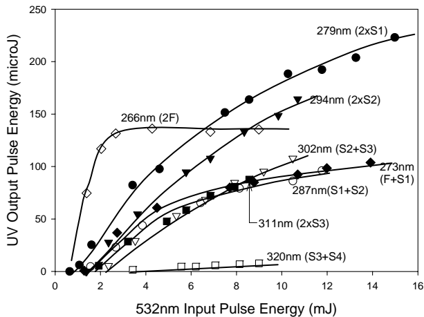
Fig. 4 Output energy at 10Hz for each UV wavelength as a function of input energy. (F = fundamental, S_n = n th Stokeses.).
