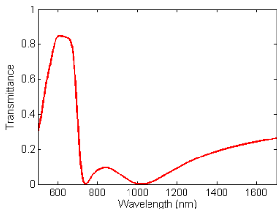
Fig. 3. Transmittance spectrum of the waveguide shown in Fig. 1(b) where w=50 nm, d=100 nm, h=200 nm, w_d=100 nm, and w_s=50 nm.
