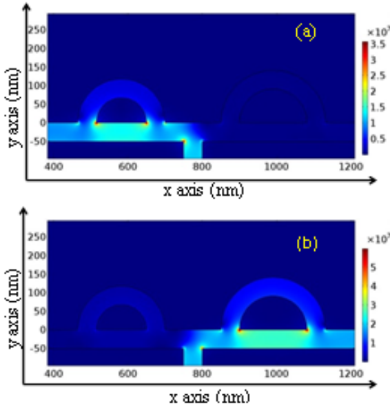
Fig. 14. Energy density inside the T-shaped waveguide for the SPPs waves with wavelengths: (a) \lambda = 570 nm, and (b) \lambda = 710 nm for the waveguide shown in Fig. 13 where w=50 nm, and the effective length of semi-circular ring shaped grooves on the left and right sides are respectively: L_{eff}=290 nm, and L_{eff}=364 nm.
