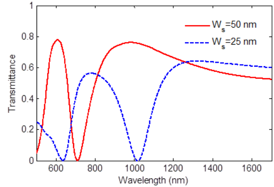
Fig. 7. Transmittance spectra of the waveguide shown in Fig. 1(a) for w_s=25 nm and w_s=50 nm where d=100 nm, L_{eff}=300 nm, and w=50 nm.
