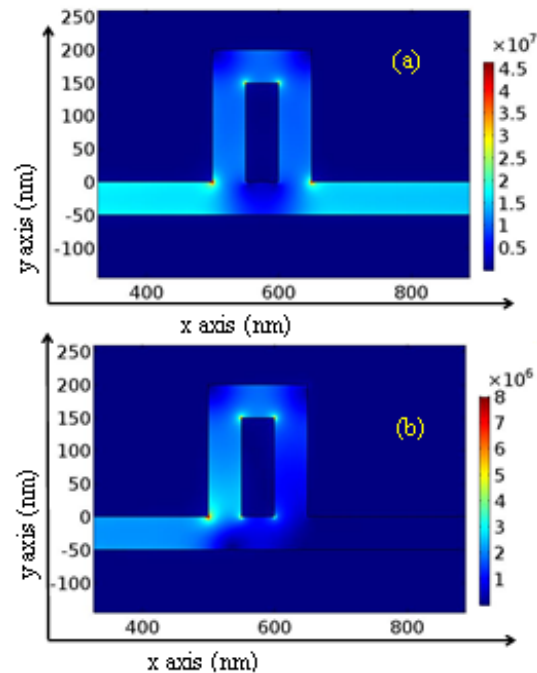
Fig. 5. Energy density inside the waveguide shown in Fig. 1(b) where w=50 nm, d=100 nm, h=200 nm, w_d=100 nm, and w_s=50 nm for the wavelengths: (a) \lambda=610 nm, and (b) \lambda=738 nm.
