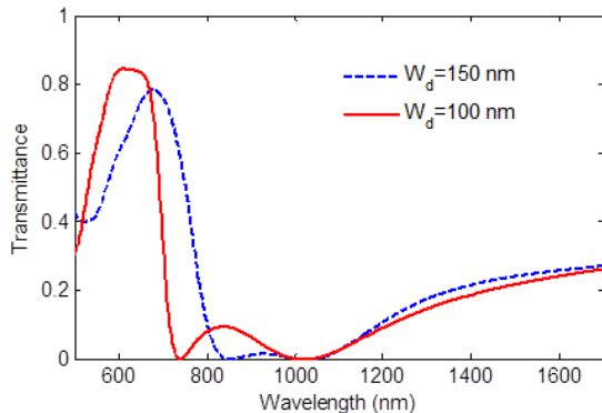
Fig. 9. Transmittance spectra of the waveguide shown in Fig. 1(b) for w d =100 nm, and w d =150 nm, where d=100 nm, w=50 nm, w s =50 nm, and h=200 nm.
