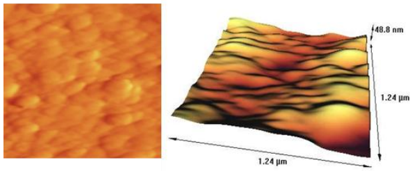
Fig. 7: AFM 3D (right) and 2D (left) images of an area of about 1.5 \mu\text{m}^2 of the taper after silver deposition.
