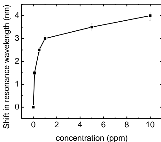
Fig. 10: The SPR wavelength shift versus concentration of lead in water.
