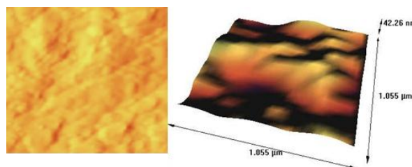
Fig. 6: Recorded 3D (right) and 2D (left) images of an area of about 1 \mu\text{m}^2 of the taper by AFM.
