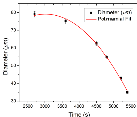
Fig. 5: Acidic etching rate of a multimode glass fiber (core/cladding-50/125 \mu\text{m} ) using HF acid with 49% purity when a 10 \mu\text{l} iters droplet is used.
