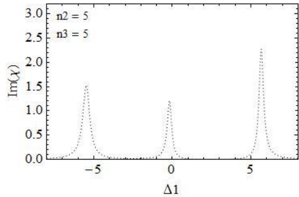
Fig. 3. Absorption spectrum of probe field versus detuning for an IYT atomic system in n_2 = 5, n_3 = 5 , \gamma_1 = \gamma_2 = \gamma_3 = 0.2\gamma , \gamma_4 = 5 \times 10^{-3}\gamma , \Delta_2 = \Delta_3 = 2.5\gamma , g_2 = g_3 = 1.5\gamma .
