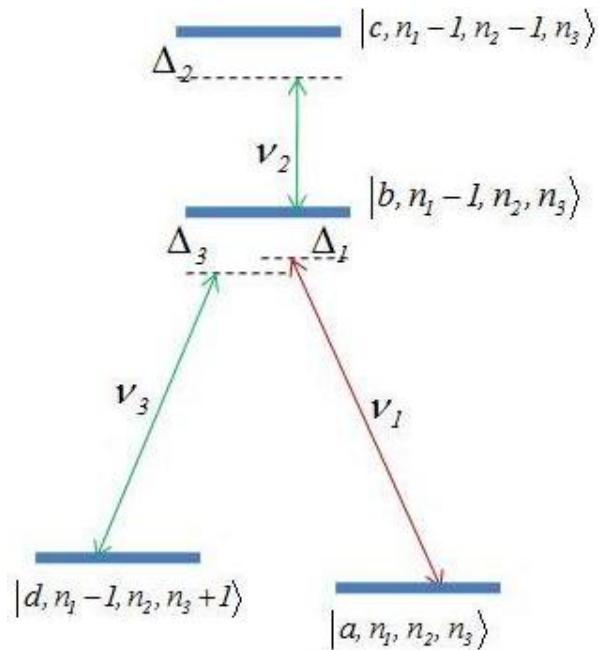
Fig. 1. Four-level IYT atomic system. The probe photon transition is shown by a red arrow. The atom-photon state is initially |a, n_1, n_2, n_3\rangle . The upper states spontaneously decay into the lower states. In this case, the decay rates for the transitions |b\rangle \rightarrow |a\rangle , |c\rangle \rightarrow |b\rangle , |b\rangle \rightarrow |d\rangle , and |d\rangle \rightarrow |a\rangle are 2\gamma_1 , 2\gamma_2 , 2\gamma_3 , and 2\gamma_4 .
