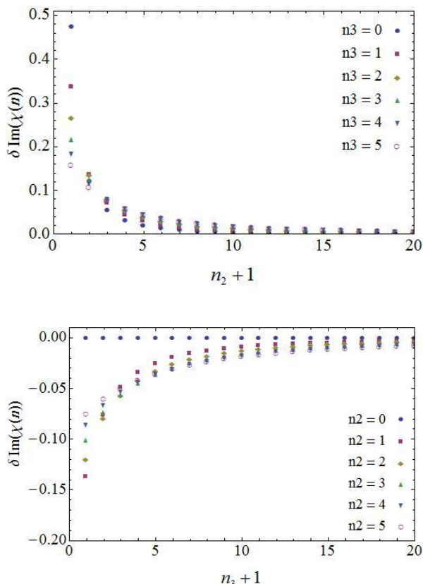
Fig. 10 The difference of absorption for neighbor peaks versus the different number of coupling photons, where the coupling fields are in the resonance condition. The parameters are similar to those chosen in Fig.3.
