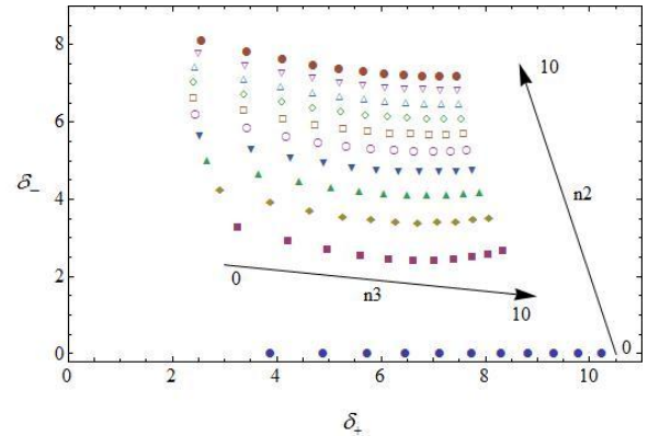
Fig. 11. Variation of \delta_+ and \delta_- for different numbers of coupling fields n_2 = (0,1,2,...10) and n_3 = (0,1,2,...10) in a four level IYT atomic system, where the parameters are the same as those chosen in Fig. 3.
