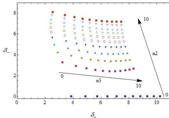
Fig. 11. Variation of \delta_+ and \delta_- for different numbers of coupling fields n_2 = (0,1,2,...10) and n_3 = (0,1,2,...10) in a four level IYT atomic system, where the parameters are the same as those chosen in Fig. 3.
