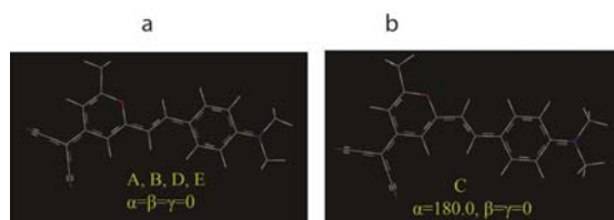
Fig. 5. (a), cis isomer and (b), trans isomer. Geometry minimizations have been performed at PCM-B3LYP/6-31G(d) level.
