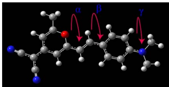
Fig. 1. [2-[2-[4-(dimethylamino)phenyl]ethenyl]-6-methyl-4H-pyran-4-ylidene]-propanedinitrile (DCM). \alpha , \beta and \gamma are the three rotors (dihedral angles) used to investigate for potential energy curves (PECs) on ground ( S_0 ) and first excited ( S_1 ) states. This picture has been depicted by gaussview 05 software.
