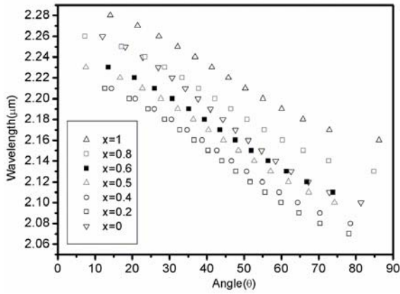
Fig. 3 Calculated phase-matching angles in YZ principle plane for LiGa(Se x S 1-x ) 2 (0 < x < 1) nonlinear crystals at \lambda_p=1064\text{nm} .
